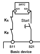
Fig. 3: Feedback loop
