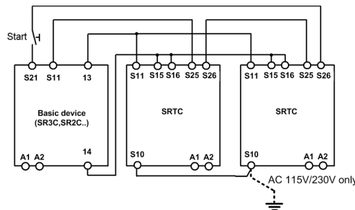
Fig. 3: Feedback loop
