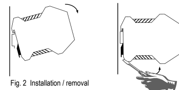
Fig. 2 Installation / removal
