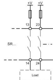
Fig. 6: Connecting load to safety contacts.
