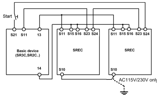
Fig. 2: Connection of several SREC Units to Basic Device
