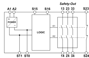
Fig. 1 Block diagram SREC
