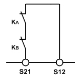
Fig. 7: Feedback loop for automatic start: The feedback loop monitors contactors or the expansion modules.
