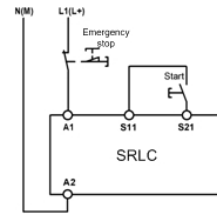
Fig. 2: Single-channel emergency stop circuit without fault monitoring of the emergency stop button and the supply cables. (up to category 1, PL c)
