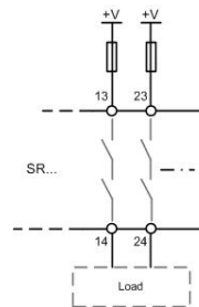
Fig. 9: Connecting load to safety contacts. (Figure shows example. Voltage „+V“ according to techn. Data)
