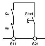
Fig. 6: Feedback loop for monitored manual start: The feedback loop monitors contactors or the expansion modules.
