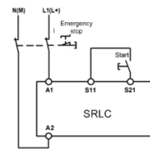
Fig. 1: Two-channel emergency stop circuit without fault monitoring of the emergency stop button and the supply cables. (up to category 3, PL d)
