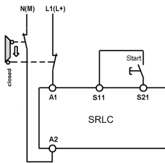
Fig. 3: Two-channel sliding guard monitoring with positively driven limit switches. (up to category 3, PL d)
