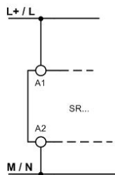
Fig. 8: Power supply A1 and A2. (Power supply according to techn. Data)
